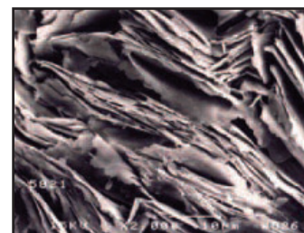
Vermiculite's thin, flexible, soft plates can be exfoliated like graphite. They retain the sealability and low porosity of graphite, but Flexitallic's Thermiculite® sheet gaskets will not oxidise at high temperatures.
